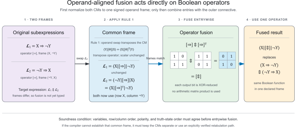
Figure 2: Two operator occurrences are first rewritten into one declared operand frame and are then fused entrywise. The transformed bra–operator–ket expression records the operand exchange explicitly; fusion is not applied while the frames differ.
