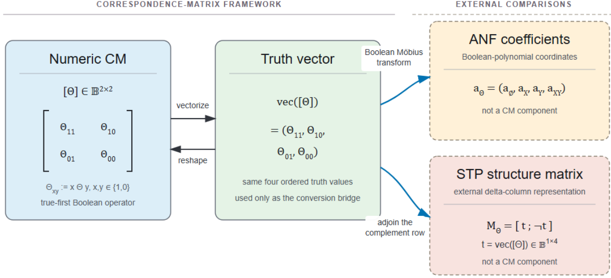
Figure 3: Numeric representation boundaries. Vectorization exposes the ordered truth values used to compare a CM with ANF coordinates and an STP logical structure matrix. ANF and STP are external representations rather than CM components. The symbolic LM path is shown separately in Figure 4.
