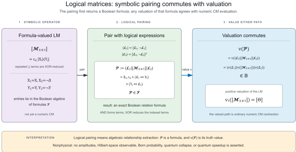
Figure 4: A formula-valued LM is paired with logical expressions before or after valuation. Because valuation is a Boolean-algebra homomorphism, both paths give the same truth value. Logical pairing denotes algebraic relationship extraction, not a physical measurement process.
